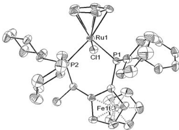
Figure 4. ORTEP diagram of ( R )- 6 . Thermal ellipsoids are drawn to 50% probability level. Hydrogen atoms are omitted for clarity. Selected bond parameters: \Delta = 0.037(4) Å; \text{HA} = 2.22^\circ ; \text{C}^*-\text{Ru1} 1.858(4) Å; \text{Ru1}-\text{P1} 2.2804(11) Å; \text{Ru1}-\text{P2} 2.3115(11) Å; \text{Ru1}-\text{Cl1} 2.4525(11) Å; \text{P1}-\text{Ru1}-\text{P2} 90.22(4)^\circ ; \text{P1}-\text{Ru1}-\text{Cl1} 89.22(4)^\circ ; \text{P2}-\text{Ru1}-\text{Cl1} 90.41(4)^\circ .
