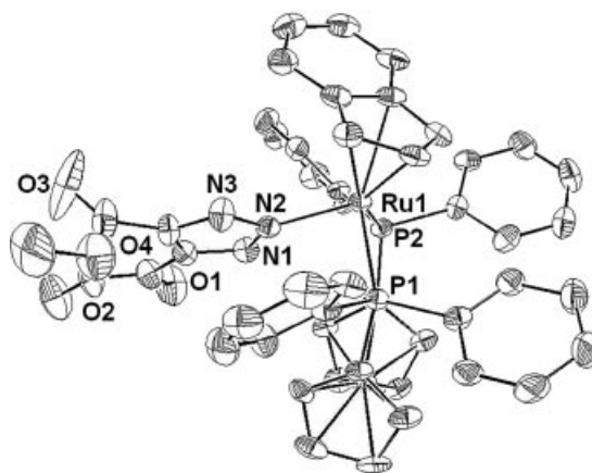
Figure 7. ORTEP diagram of 9 . Thermal ellipsoids are drawn to 50% probability level. Hydrogen atoms are omitted for clarity.
