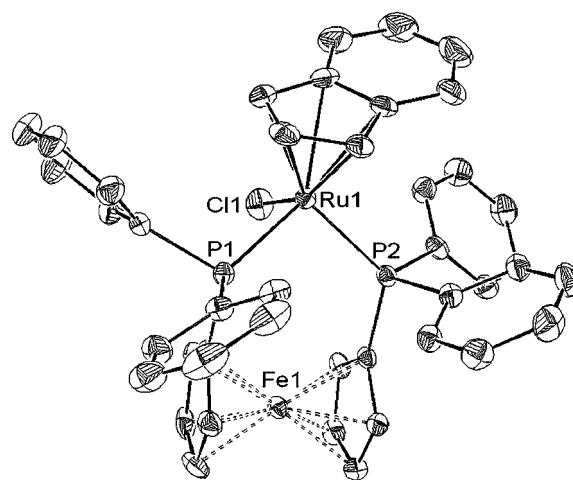
Figure 2. ORTEP diagram of 3 . Thermal ellipsoids are drawn to 50% probability level. Hydrogen atoms are omitted for clarity.
