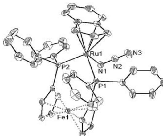
Figure 6. ORTEP diagram of 8 . Thermal ellipsoids are drawn to 50% probability level. Hydrogen atoms are omitted for clarity. Selected bond parameters: \Delta = 0.163 Å; HA = 6.85^\circ ; FA = 8.70^\circ ; C*–Ru1 1.892 Å; Ru1–P1 2.2559(5) Å; Ru1–P 22.3251(6) Å; Ru–N1 2.1355(18) Å; N1–N2 1.192(3) Å; N2–N3 1.156(3) Å; P1–Ru1–P2 97.744(19)°; P1 Ru1–N1 84.42(5)°; P2–Ru1–N1 92.14(5)°; Ru1–N1–N2 117.96(15)°; N3–N2–N1 176.6(2)°.
