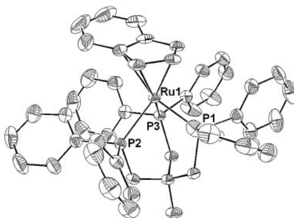
Figure 3. ORTEP diagram of [4] + . Thermal ellipsoids are drawn to 50% probability level. Hydrogen atoms are omitted for clarity.
