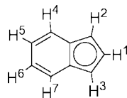
Figure 8. Numbering of indenyl protons.
