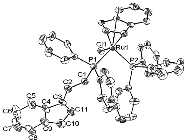
Figure 1. ORTEP diagram of 2 . Thermal ellipsoids are drawn to 50% probability level. Hydrogen atoms are omitted for clarity. Selected bond lengths: C1–C2 1.530(7) Å; C2–C3 1.506(6) Å; C3–C11 1.329(7) Å; C3–C4 1.454(7) Å; C4–C5 1.375(7) Å; C5–C6 1.388(8) Å; C6–C7 1.374(9) Å; C7–C8 1.368(9) Å; C8–C9 1.385(8) Å; C9–C4 1.401(7) Å; C9–C10 1.513(8) Å; C10–C11 1.494(7) Å. Other bond parameters are given in Table 1.
