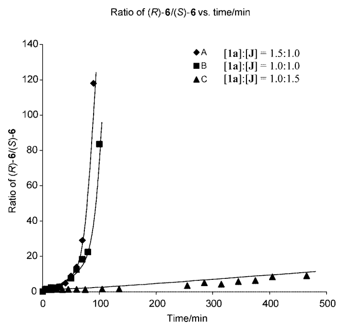
Figure 5. A plot of the ratio of ( R )- 6 /( S )- 6 vs. time for the reaction of 1a with Josiphos ( J ); [ J ] = 10 mM.
